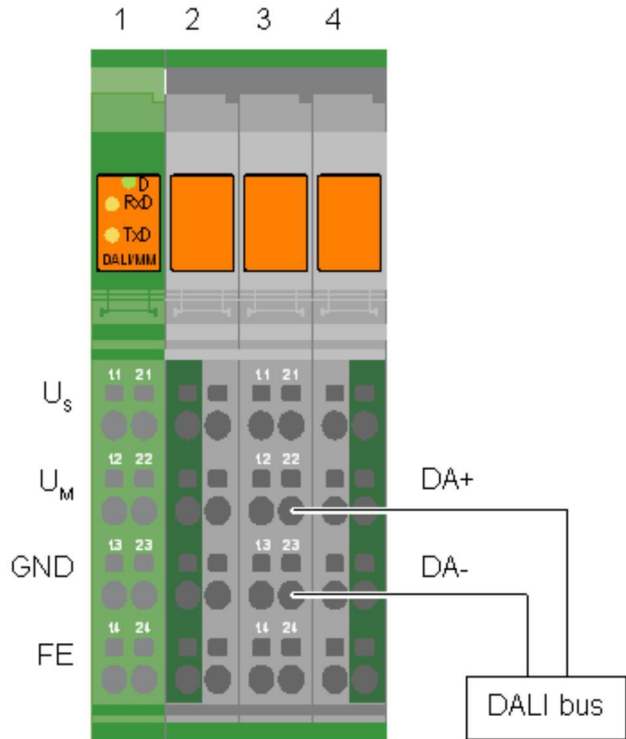
Figure 4 Connection example
