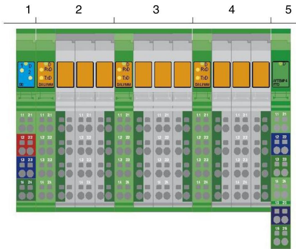
Figure 5 Typical station structure with several DALI terminals
