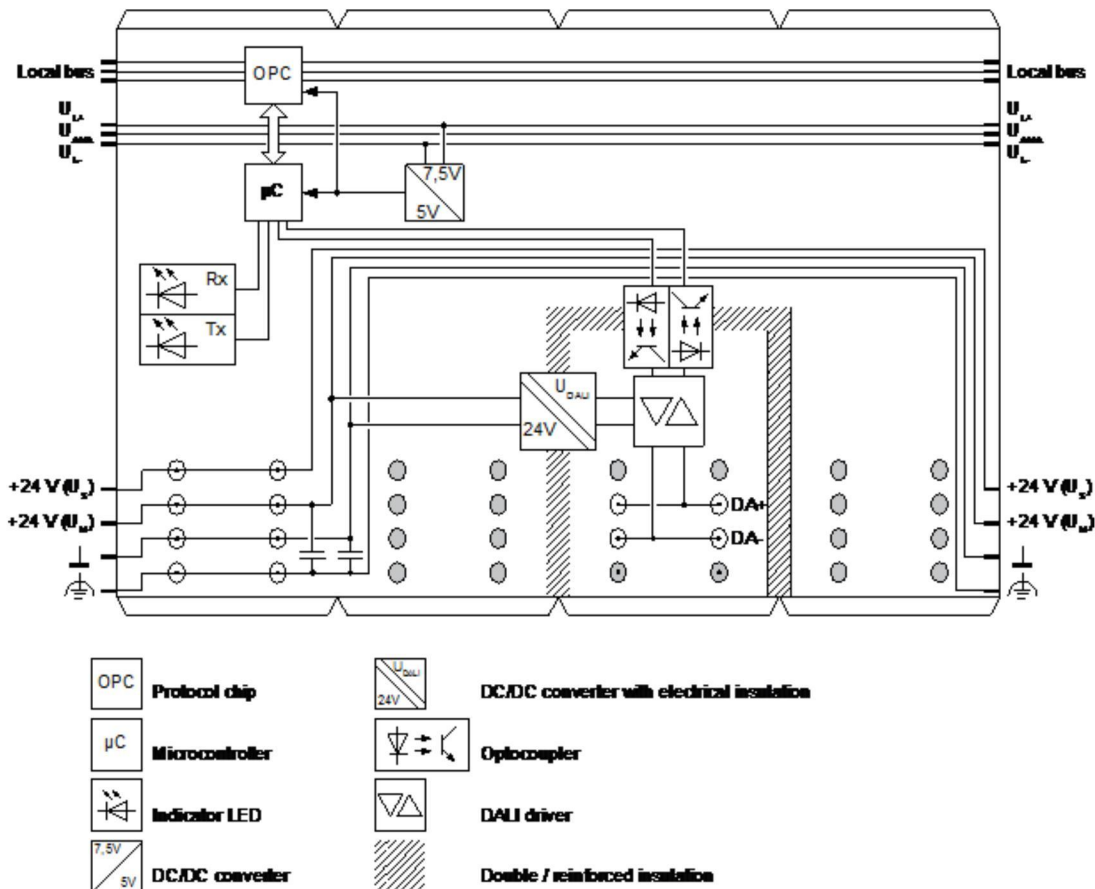
Figure 1 Internal wiring of the terminal points
